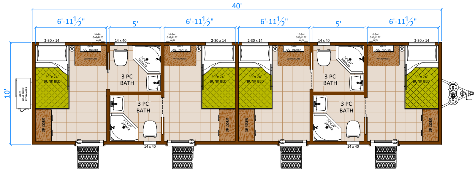
WORK FORCE 8 - SLEEPER (WF1040) (400 SQ. FT.)
