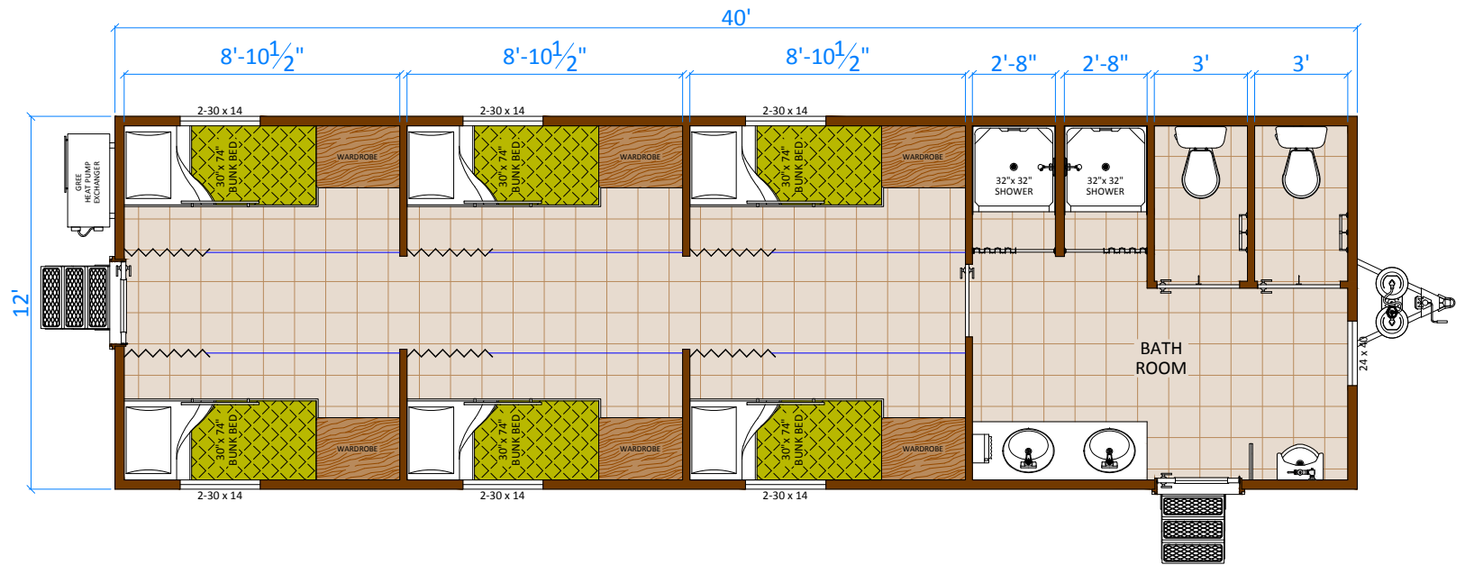
WORK FORCE 12 - SLEEPER (WF1240) (480 SQ. FT.)
