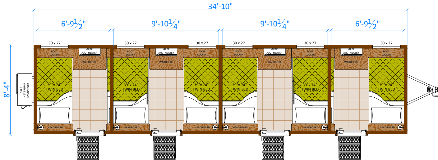
WORK FORCE 8 - SLEEPER (WF835) (290.3 SQ. FT.)
