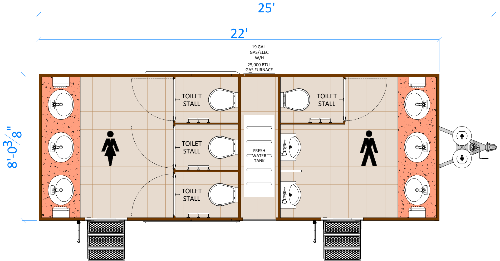
WASHROOM (W228) (176 SQ. FT.)
